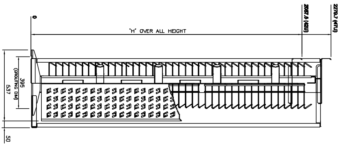
SIDE VIEW
